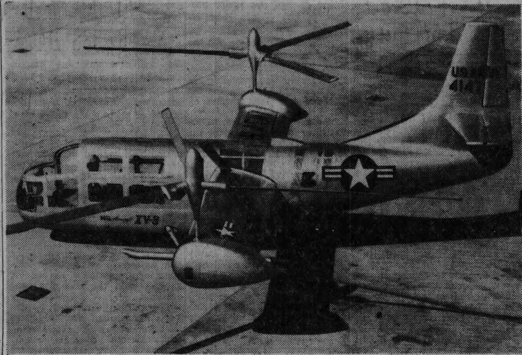
Bell Aircraft's XV-3, which can take off and land vertically and fly like a fixed-wing plane
